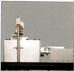
UBPS 非饱和土直剪仪 UBPS Unsaturated Back Pressured Shearbox
