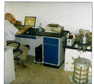
RCA 共振柱设备 RCA Resonance Column Apparatus
