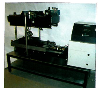
Geocomp 土和土工织物大型剪切仪 Geocomp Large Shear Apparatus for Soil and Geosynthetics Testing
